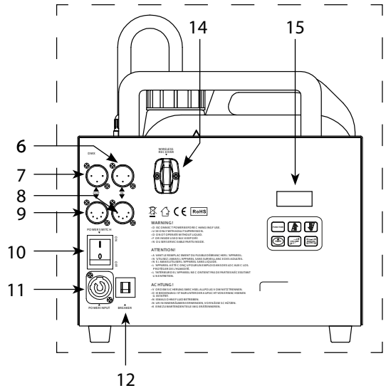
Rear panel
